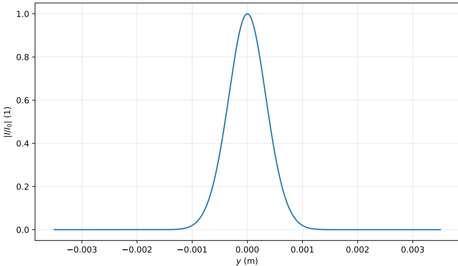
Intensity profile I(x = 0, y, z = 0.478)/I_0 , P_{in}=0.3P_{cr} , artificial time
